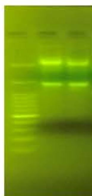
RNA structure integrity analysis
