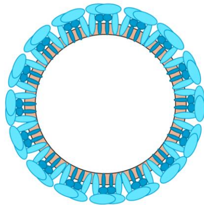
Non-infectious VLP
