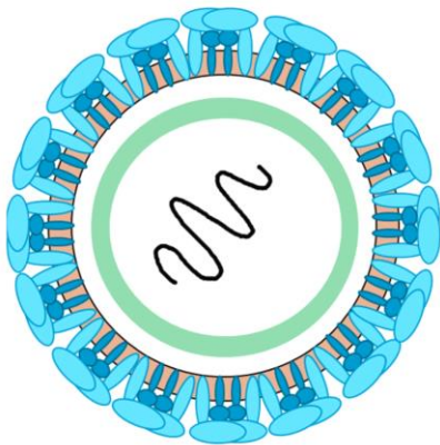
Infectious Virion
