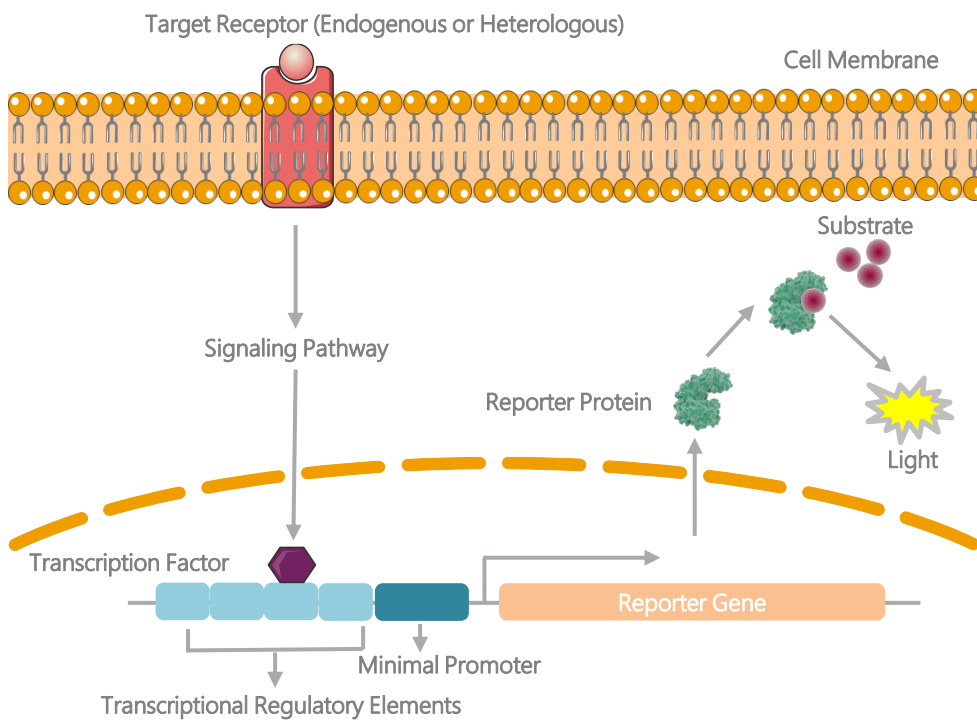
FIGURE 1 The principle of signaling pathway reporter assay
