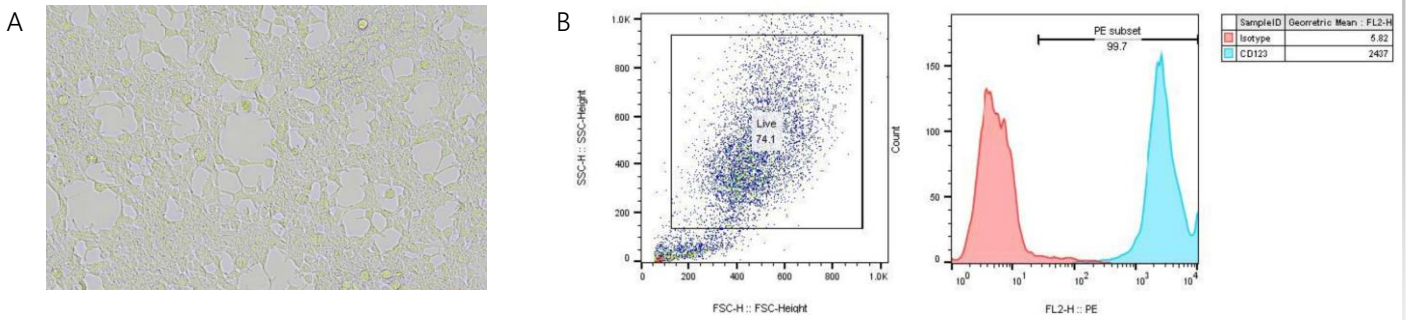
Figure 3. A: Monkey IL3RA Stable Cell Line-HEK293T; B: Flow cytometry analysis of monkey IL3RA expression in HEK293T cells.
