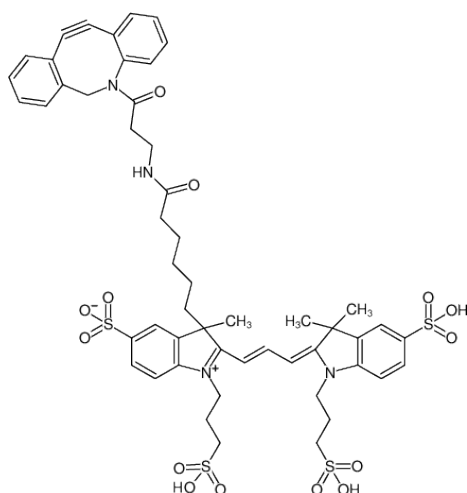
Structural formula of DBCO-AZDye555
