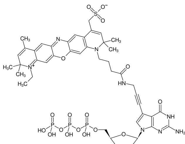
Structural formula of 7-Propargylamino-7-deaza-ddGTP-ATTO-700
